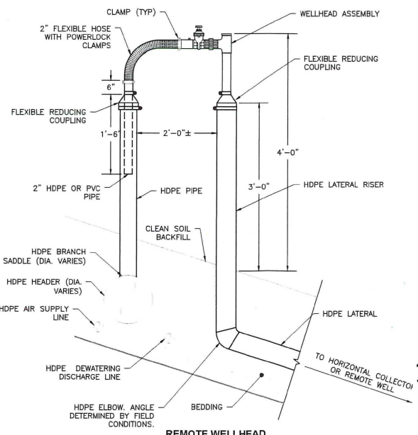
REMOTE WELLHEAD DETAIL 6 SCALE: NOT TO SCALE DS2
