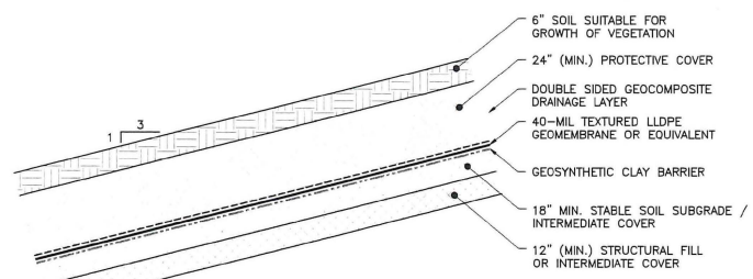
TYPICAL FINAL COVER DETAIL 4 SCALE: NOT TO SCALE DS2
