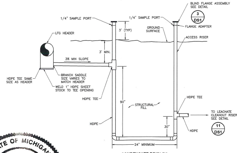
CONDENSATE DRIPLEG DETAIL 7 SCALE: NOT TO SCALE DS2
