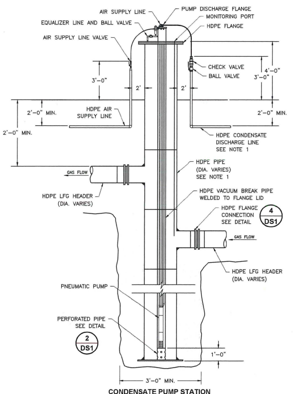
CONDENSATE PUMP STATION DETAIL 5 SCALE: NOT TO SCALE DS2
