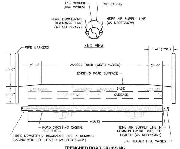
TRENCHED ROAD CROSSING DETAIL 2 SCALE: NOT TO SCALE DS2
