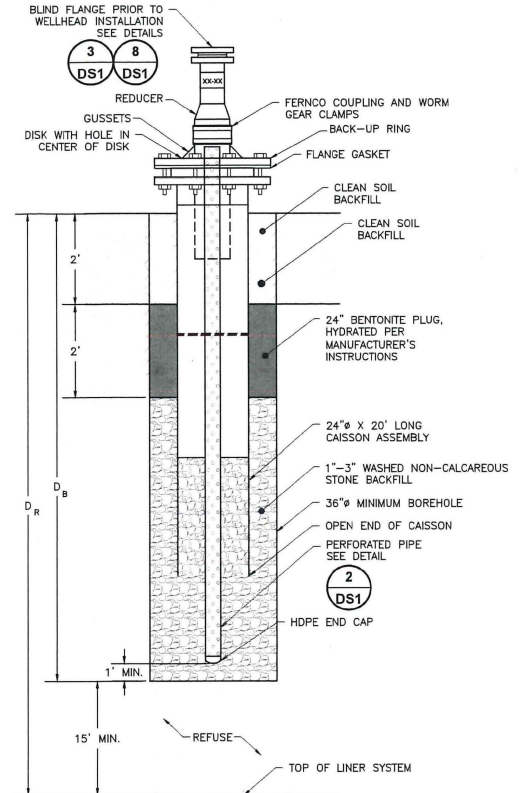
LFG EXTRACTION WELL WITH CAISSON DETAIL 3 SCALE: NOT TO SCALE DS2
