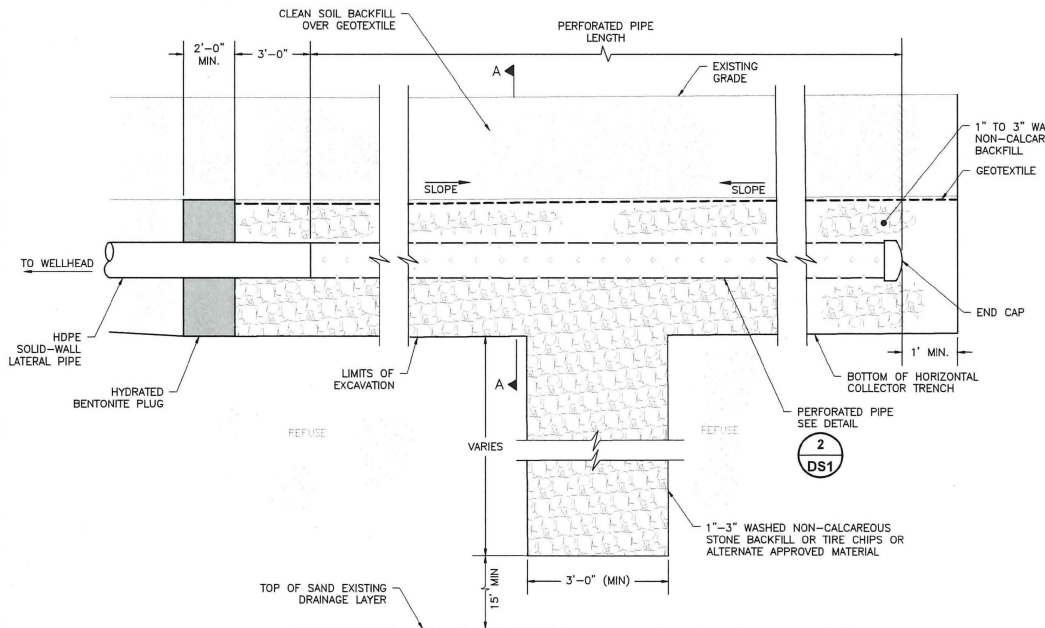
INTERIM HORIZONTAL COLLECTOR DETAIL 1 SCALE: NOT TO SCALE DS2
