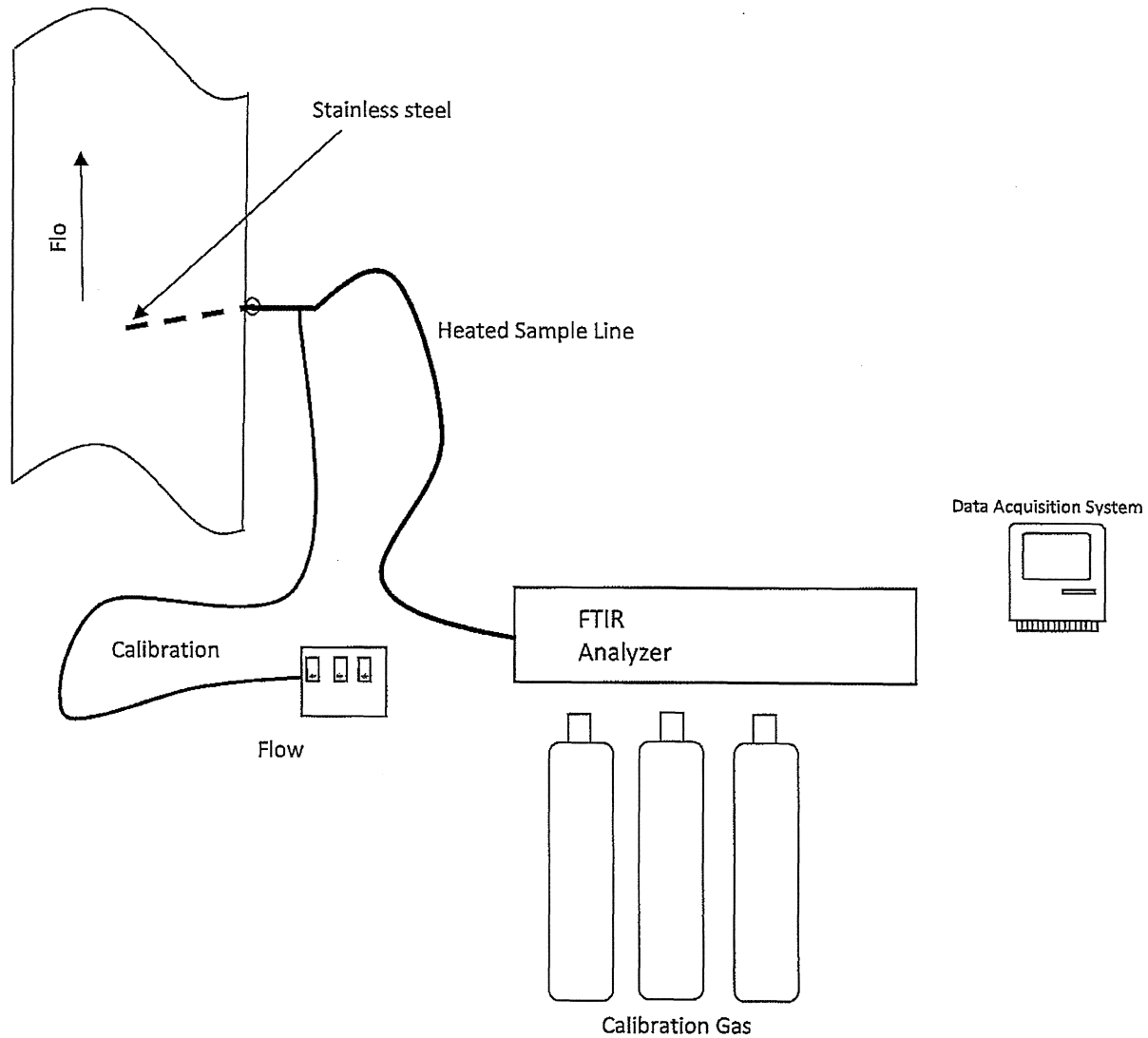
Figure 2 – ASTM D6348 Belle River Power Plant September 17-18, 2019
