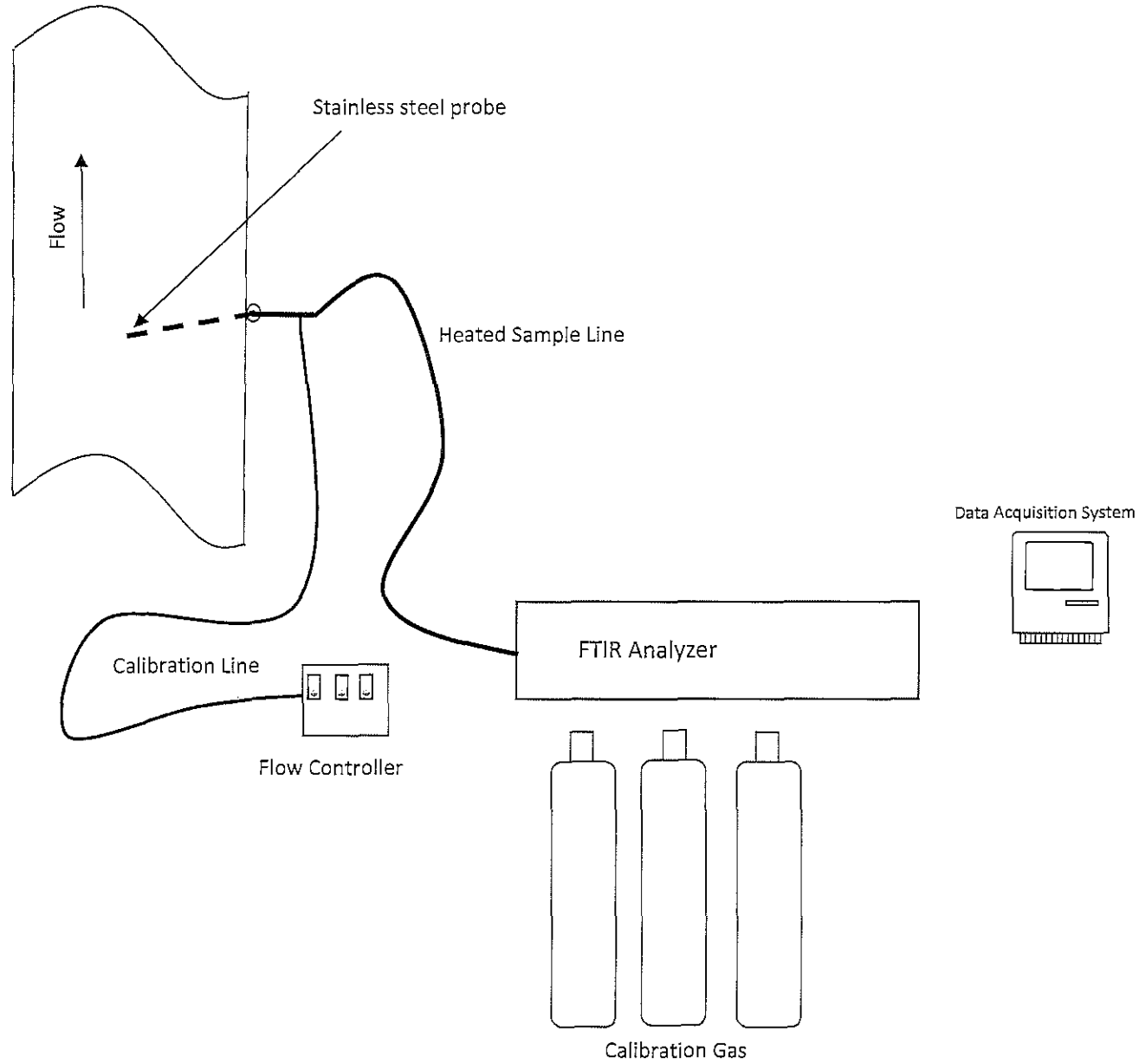
Figure 2 – ASTM D6348 St. Clair Power Plant – Unit 2 October 29, 2017
