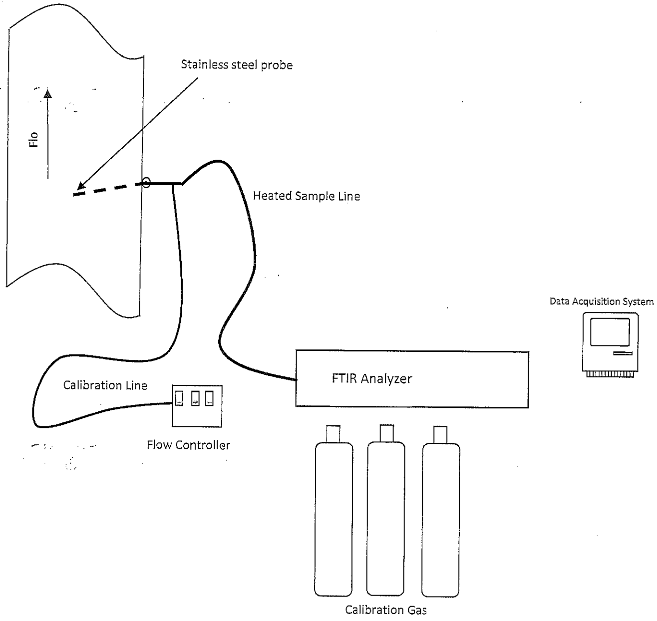
Figure 2 – ASTM D6348 Belle River Power Plant February 22, 2018
