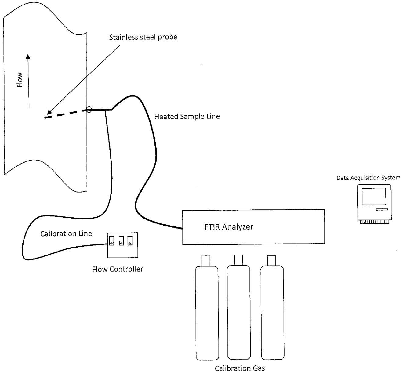
Figure 2 – ASTM D6348 St. Clair Power Plant – Unit 6 August 29, 2018
