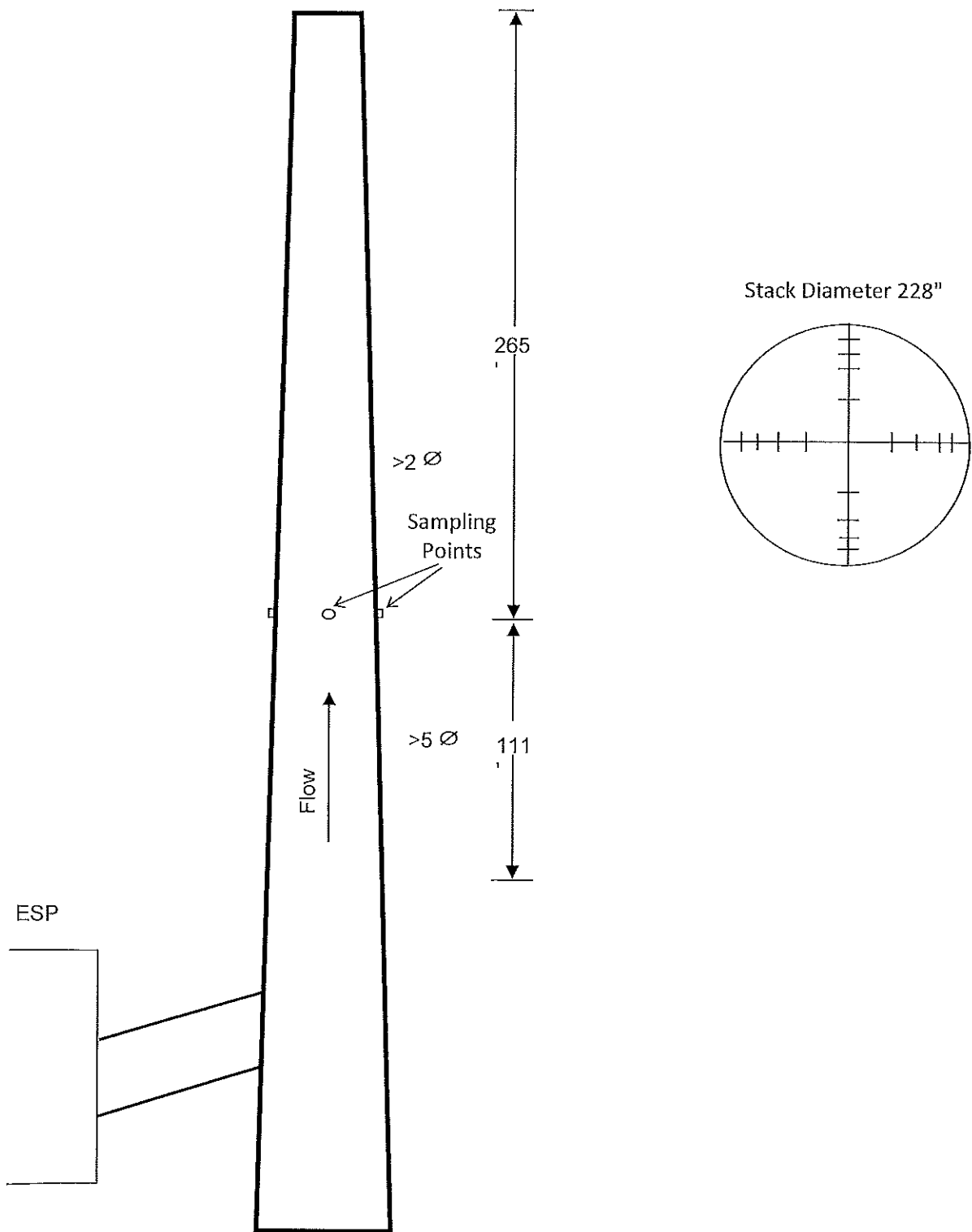
Figure 1 – Sampling Location St. Clair Power Plant – Unit 6 August 29, 2018
