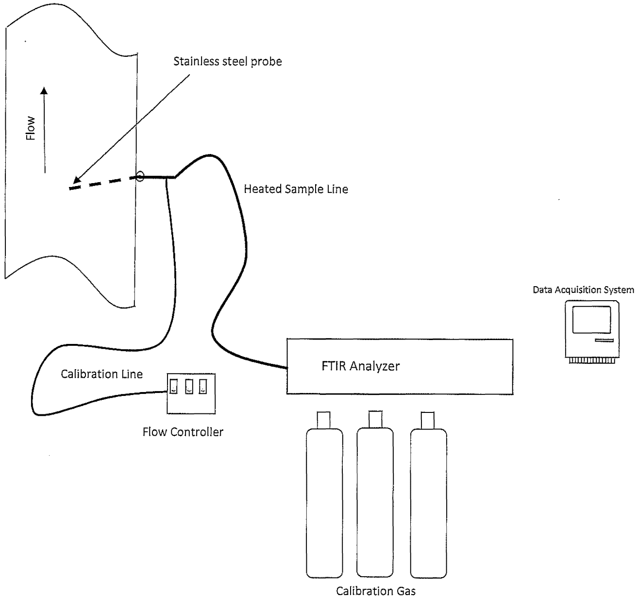
Figure 2 – ASTM D6348 St. Clair Power Plant – Unit 3 October 24, 2018
