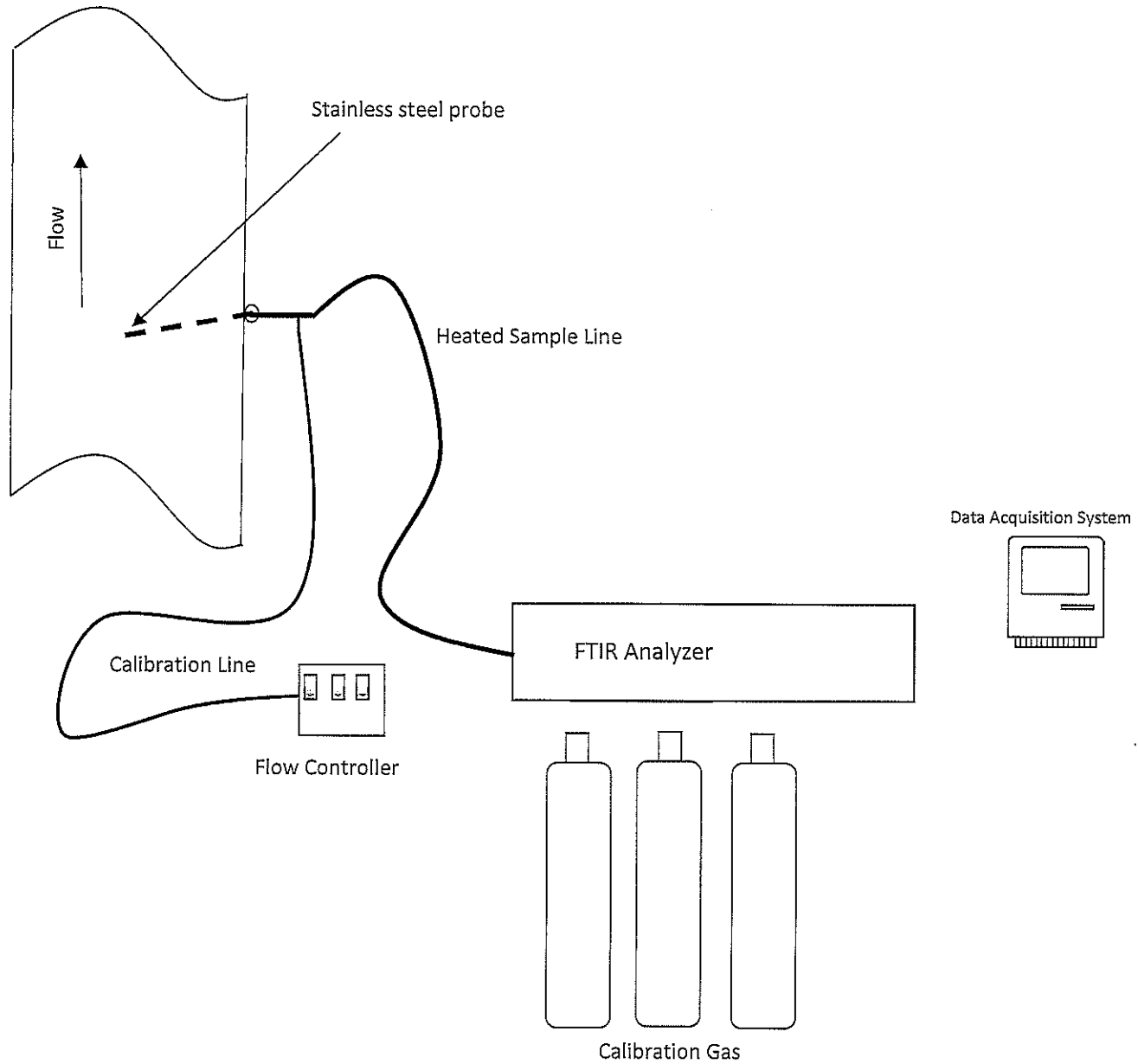
Figure 2 – ASTM D6348 St. Clair Power Plant – Unit 2 December 11, 2018
