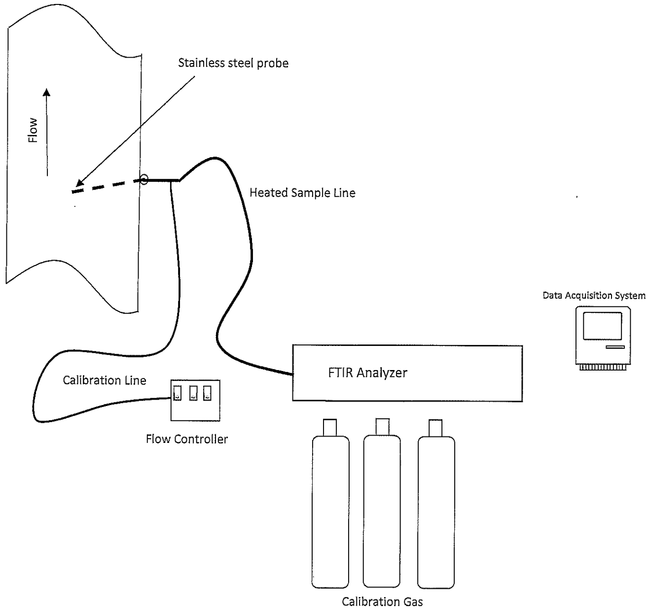
Figure 2 – ASTM D6348 St. Clair Power Plant – EU-BOILER2-SC February 28, 2019
