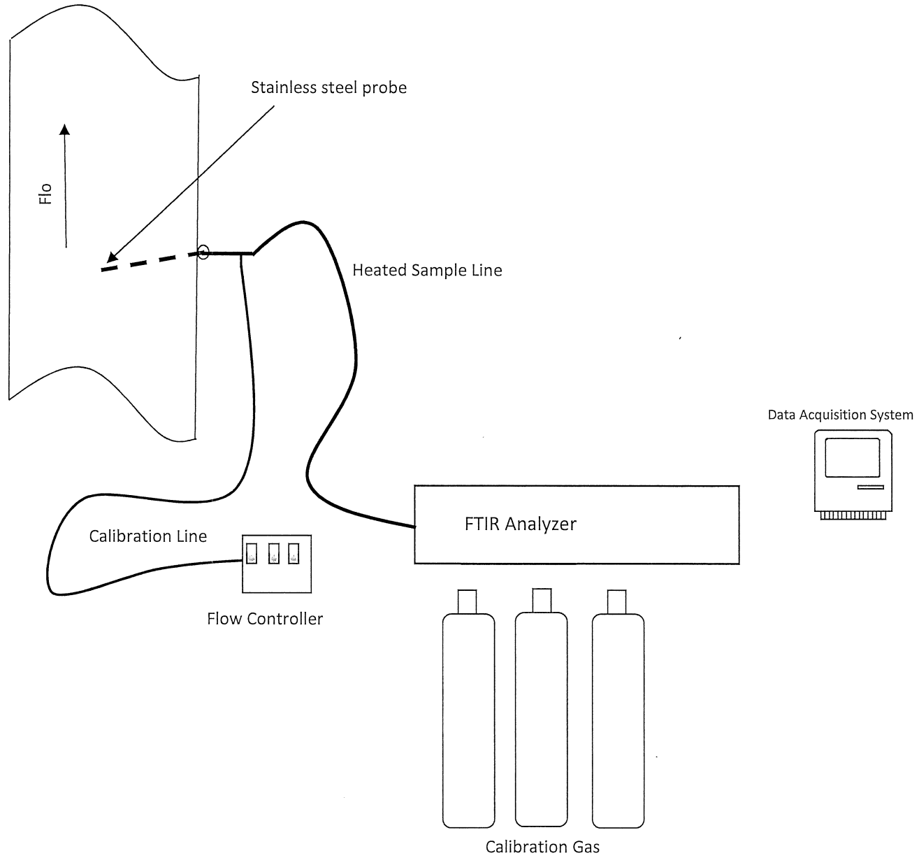
Figure 2 – ASTM D6348 Belle River Power Plant August 9, 2019
