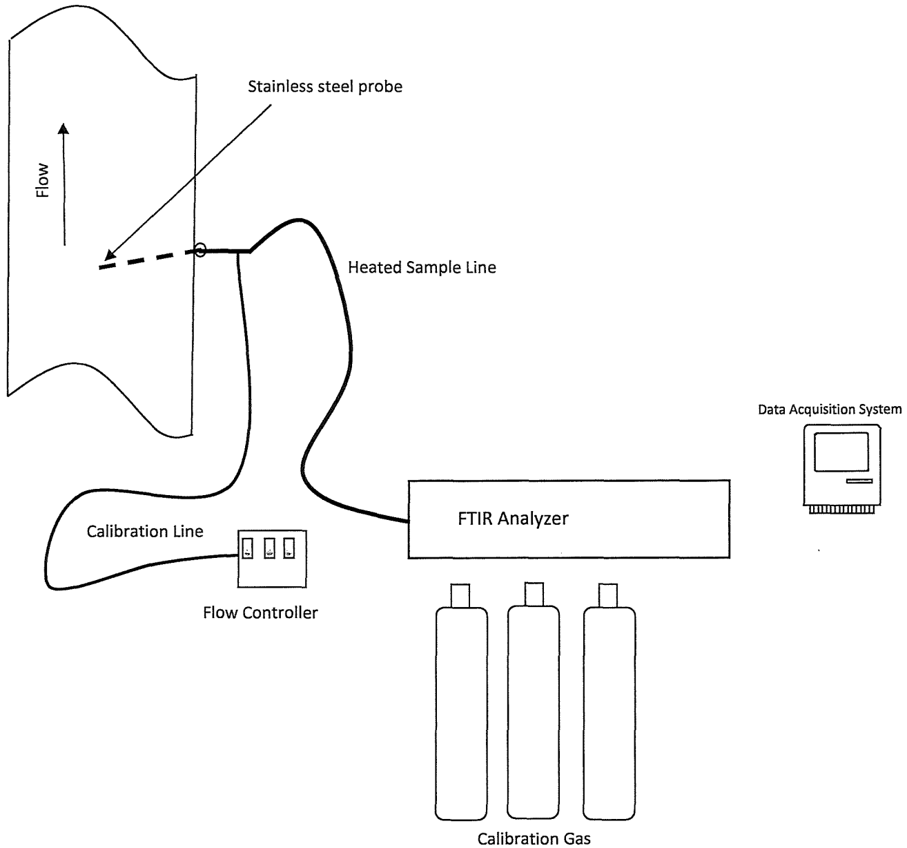
Figure 2 – ASTM D6348 Belle River Power Plant February 9, 2023
