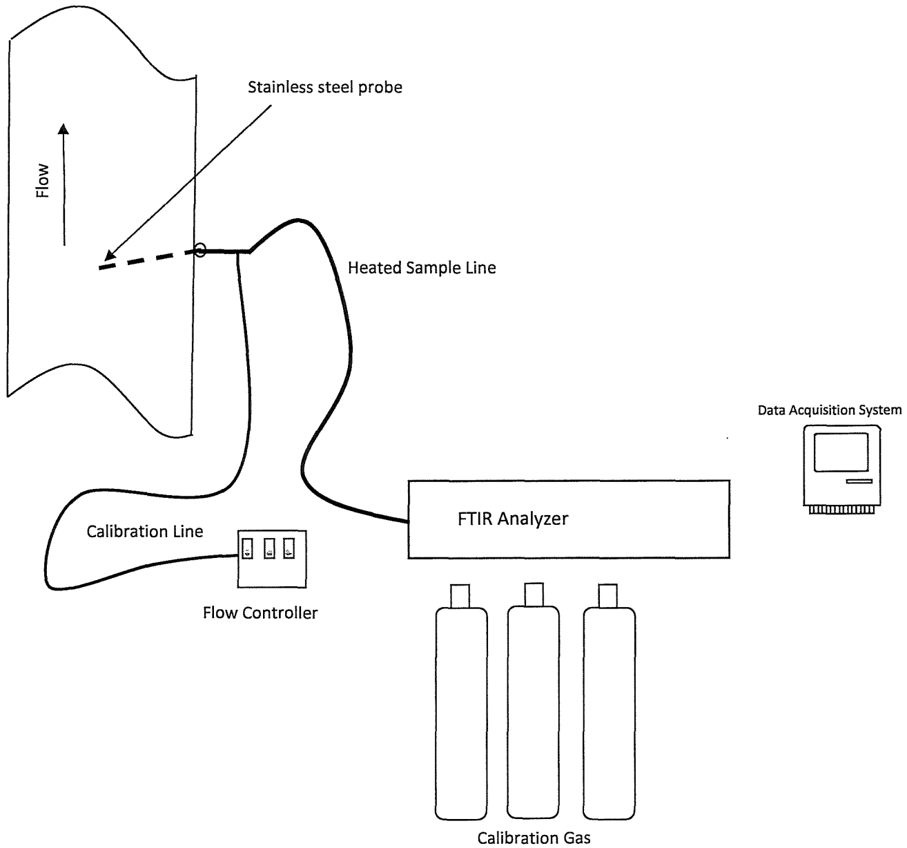
Figure 2 – ASTM D6348 Belle River Power Plant February 16, 2023
