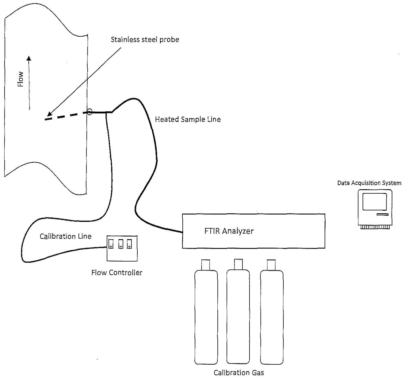
Figure 2 – ASTM D6348 River Rouge Power Plant March 23, 2018
