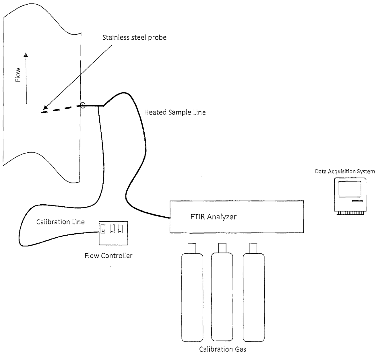
Figure 2 – ASTM D6348 River Rouge Power Plant June 6, 2018
