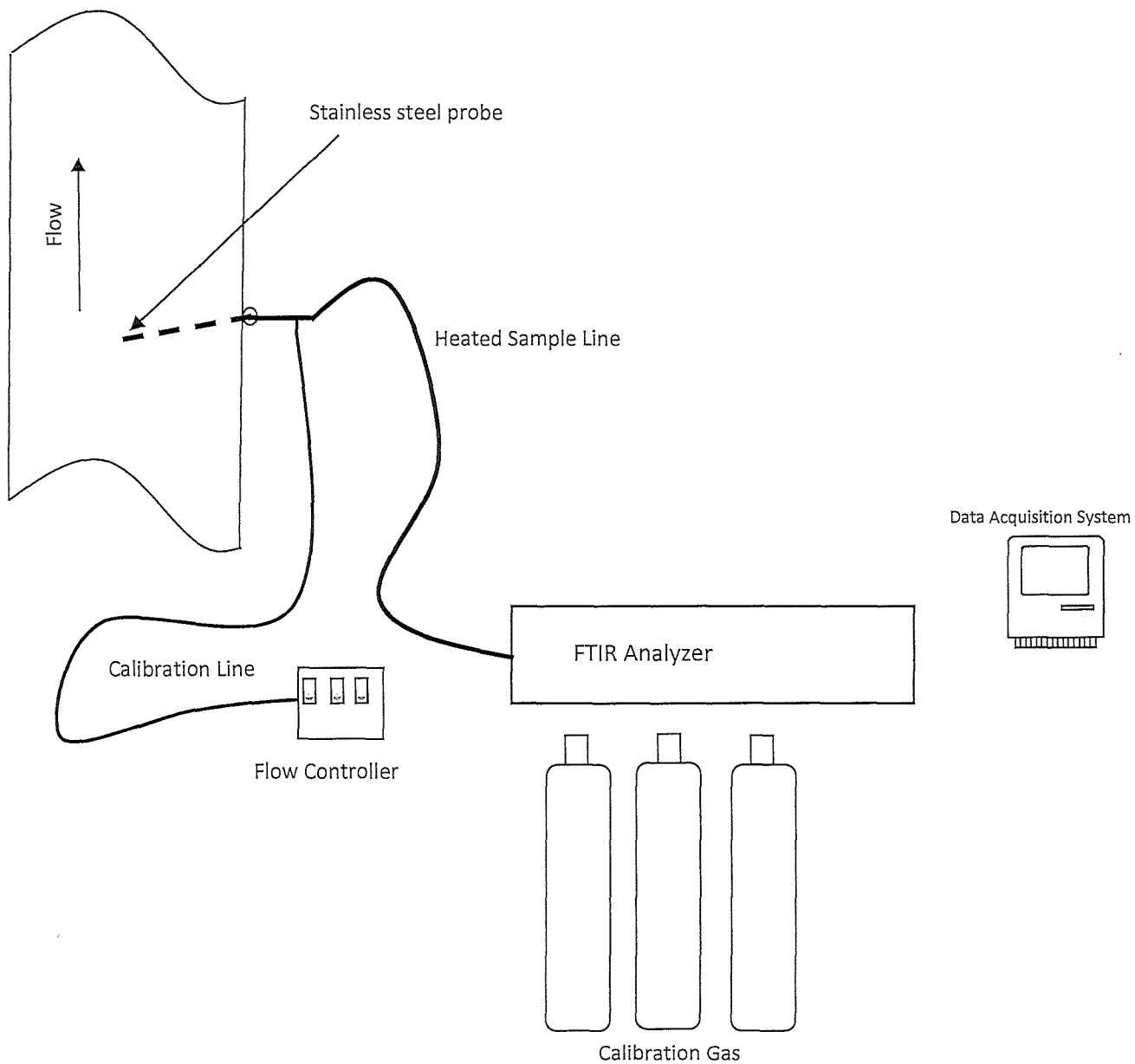
Figure 2 – ASTM D6348 River Rouge Power Plant May 28, 2020
