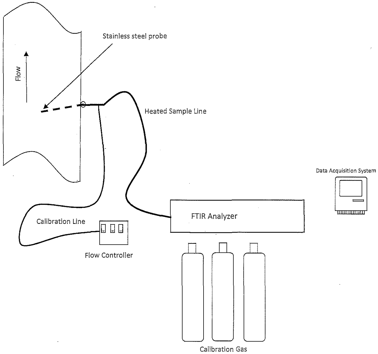
Figure 2 – ASTM D6348 Trenton Channel Power Plant August 29, 2017
