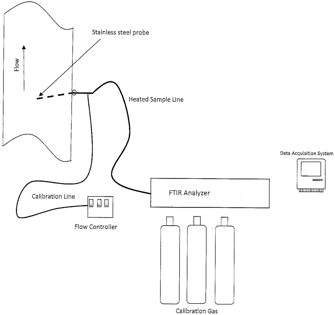
Figure 2 – ASTM D6348 Trenton Channel Power Plant March 21, 2018
