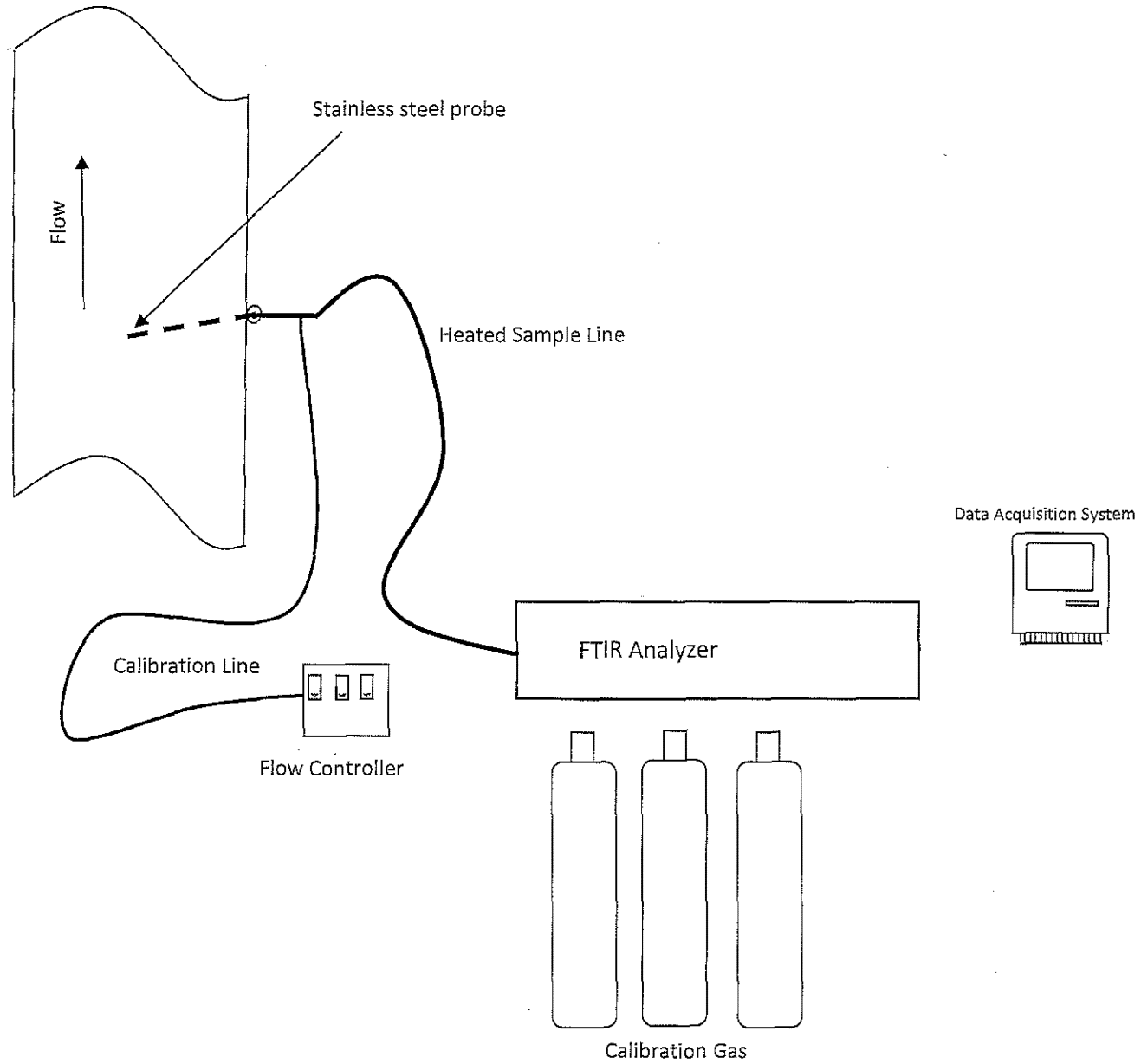
Figure 2 – ASTM D6348 Trenton Channel Power Plant September 19, 2018
