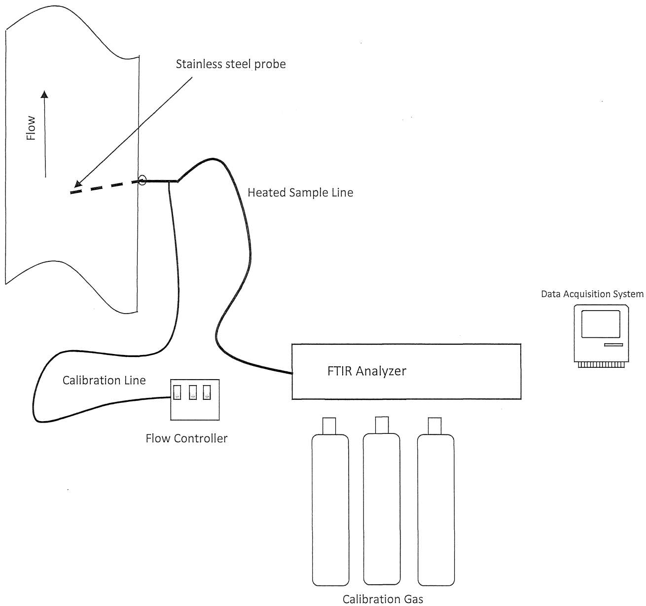
Figure 2 – ASTM D6348 Trenton Channel Power Plant September 19, 2019
