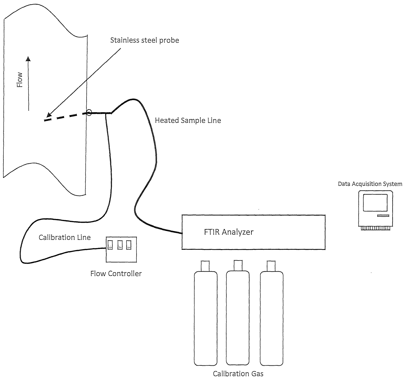
Figure 2 – ASTM D6348 Trenton Channel Power Plant June 25, 2020
