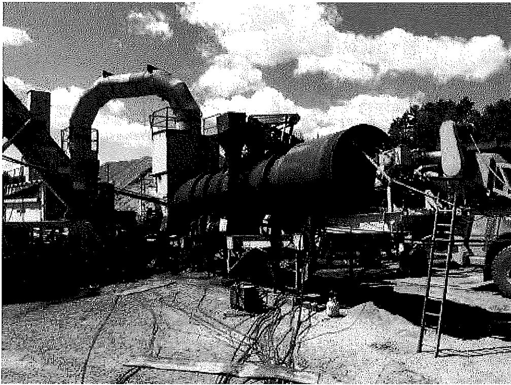
Image 1(B121) : Bacco portable asphalt plant #12
