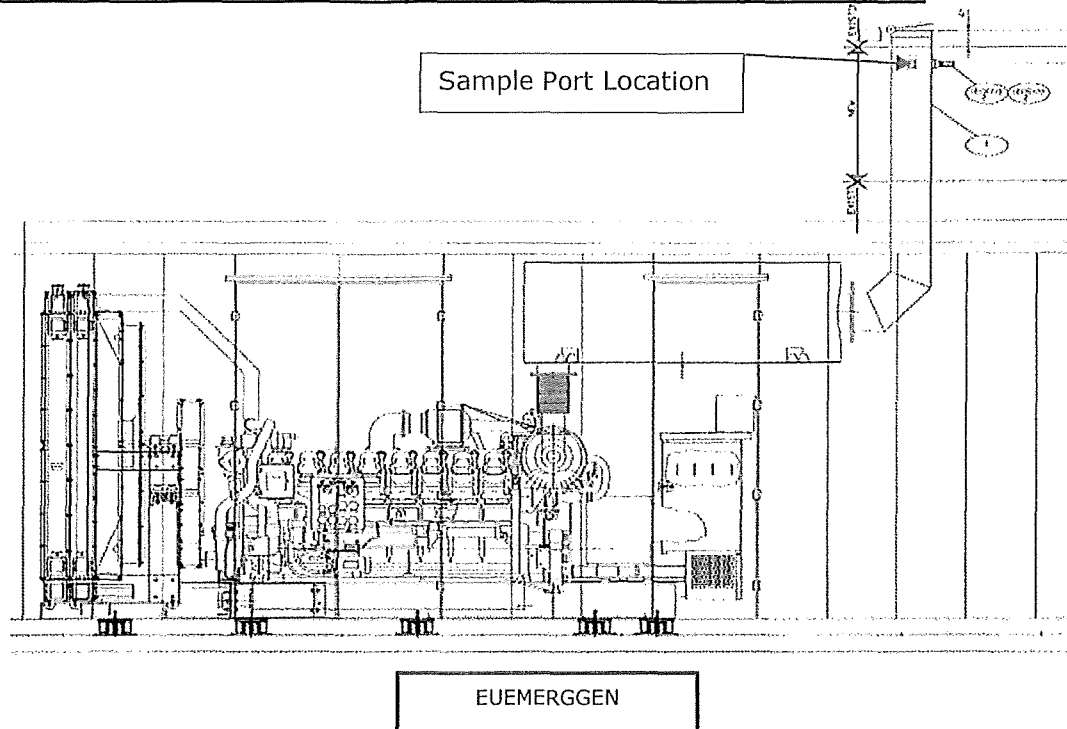
Figure 4-1. EUEMERGGEN Caterpillar Model G3512B Engine Diagram
