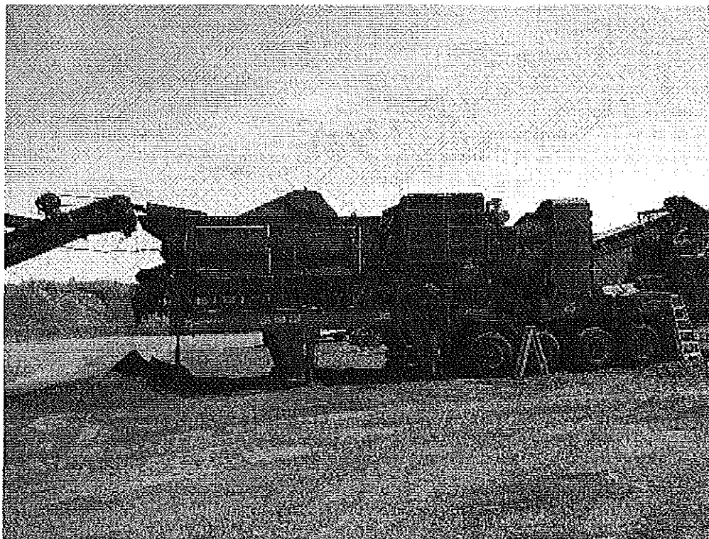
Image 2(2014 2) : Secondary jaw crusher
