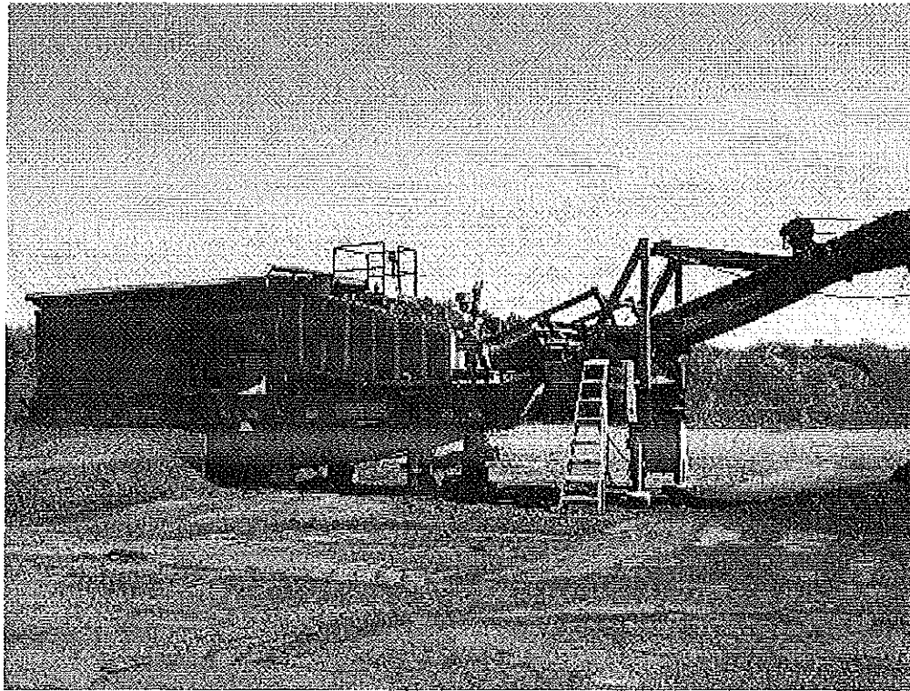
Image 1(2014 1) : Primary jaw crusher--1000
