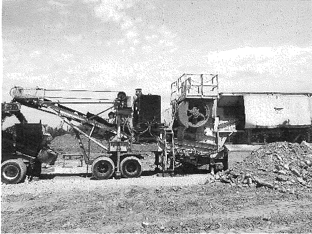
Image 6(NS6) : Screen and conveyors
