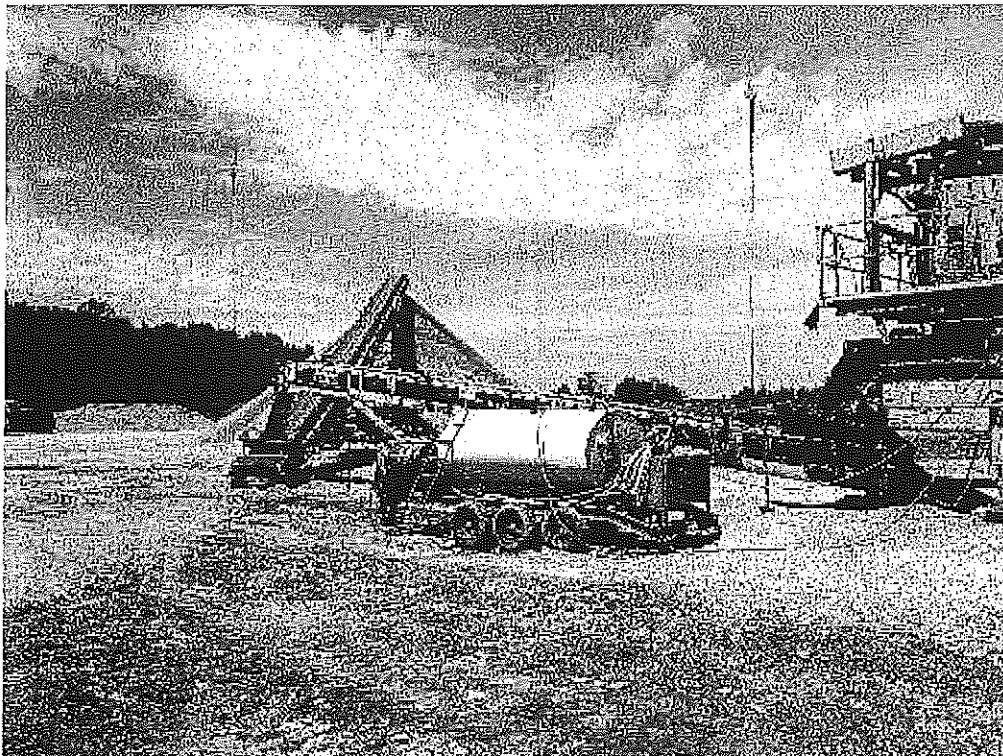
Image 3(NS3) : 1000 gallon water tank/trailer. Conveyor EU_2 is behind the water tank.
