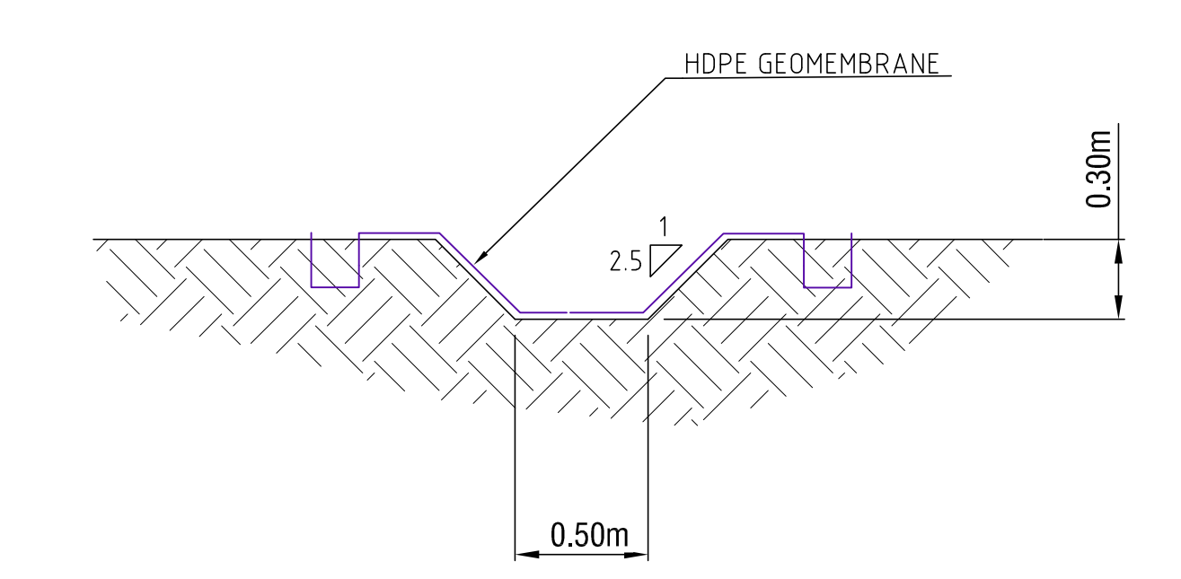
2 TYP. CONTACT WATER DITCH SECTION N.T.S.
